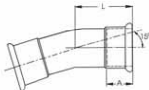
15° FF Elbow
