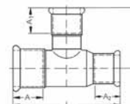
Reduced tee
