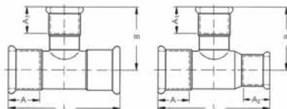
Reduced tee
