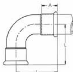
90° F.F. Short Elbow R=1D
