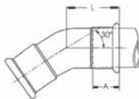
30° F.F. Elbow R=1,5D
